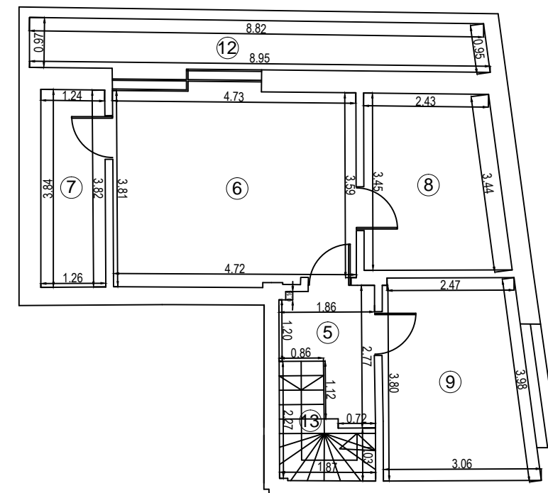
MANSARDA
